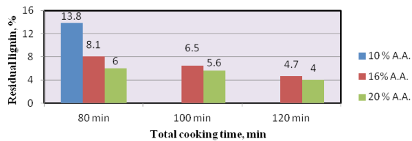
Fig.6: Influence of the cooking time and the active alkali content (A.A.) on the residual lignin in the pulp obtained from OSB.
