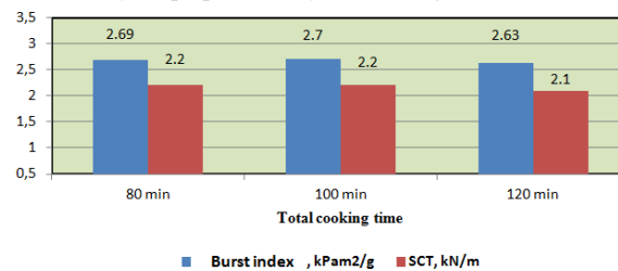
Fig.11: Burst index and SCT of the pulp obtained from disintegrated OSB at the 16 % alkali content.
