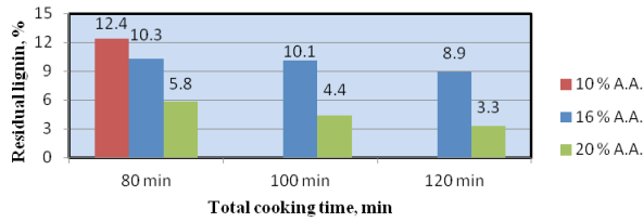
Fig.3: Influence of the cooking time and the active alkali content (A.A.) on the residual lignin in the pulp obtained from PB.
